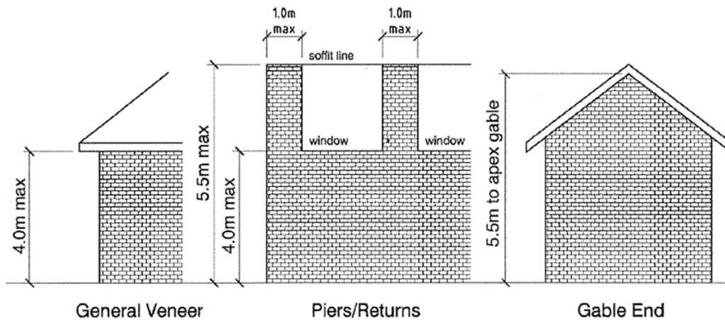
Figure 1 – Maximum veneer heights for single storey, running-bonded construction – diagram sourced from Clay Brick & Paver Manufactures association
