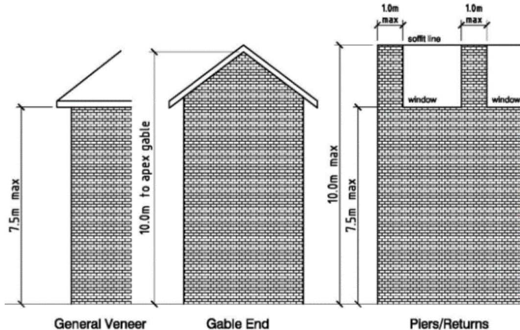
Figure 1 – Maximum Veneer Heights for two-storey stack bond construction – diagram sourced from Clay Brick & Paver Manufactures association
