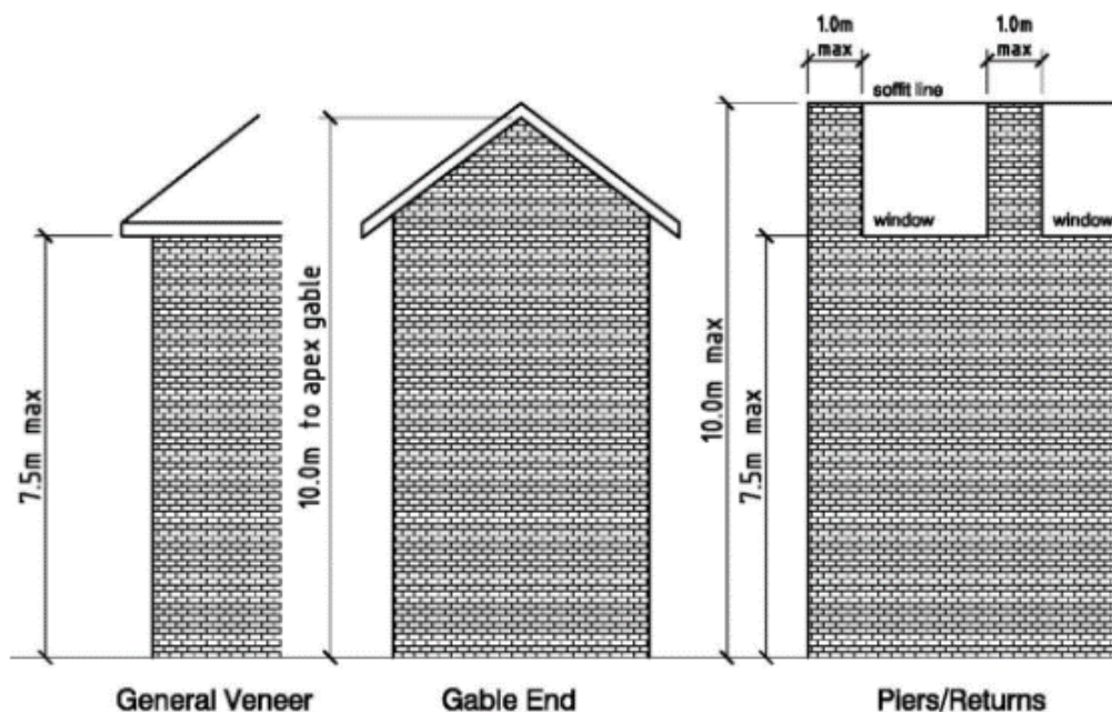
Figure 1 – Maximum Veneer Heights for two-storey running bond construction– diagram sourced from Clay Brick & Paver Manufactures association
