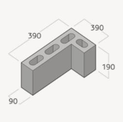
390 Corner
