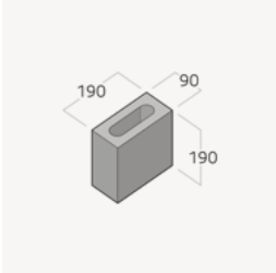
190 Standard
