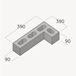
390 Half Corner
